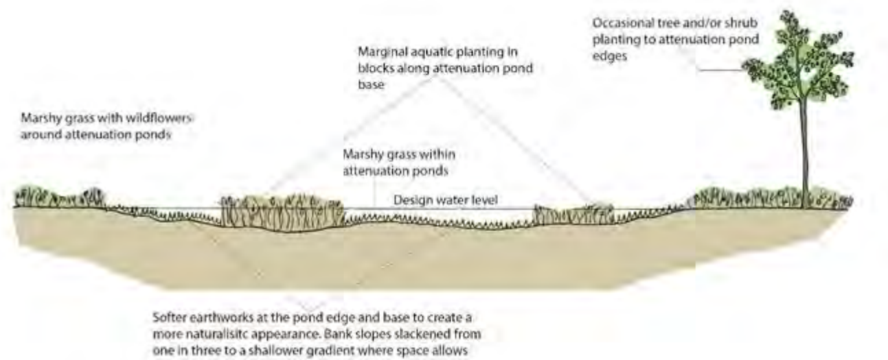
Figure 6 Indicative cross section of relatively dry attenuation pond
