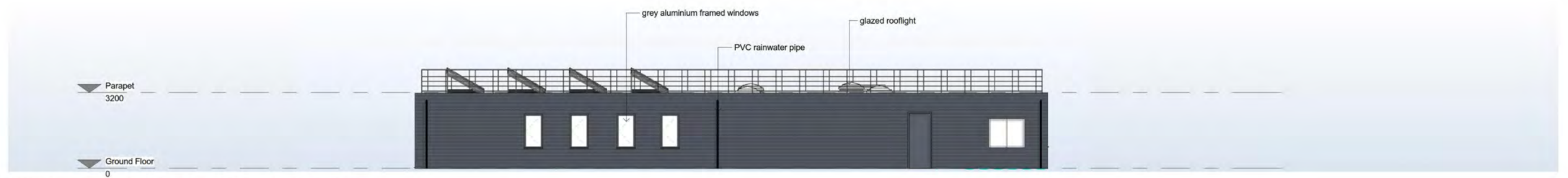
OFFICE/WELFARE BUILDING - EAST ELEVATION
